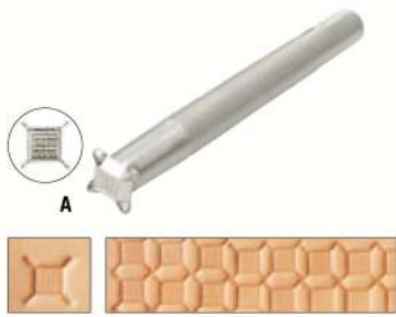
A STAMP, GEOMETRIC PATTERN With this geometric stamp, you can emboss attractive background patterns on leather. Dimensions 11,5 x 11,5 mm. Overall length 110 mm No. 708105
