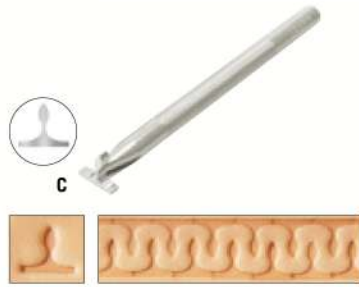
C STAMP, WAVY BORDERS With this stamp, you can emboss wavy edges and borders on leather. Closed contours are also possible. Dimensions 10 x 9 mm. Overall length 110 mm No. 708101
